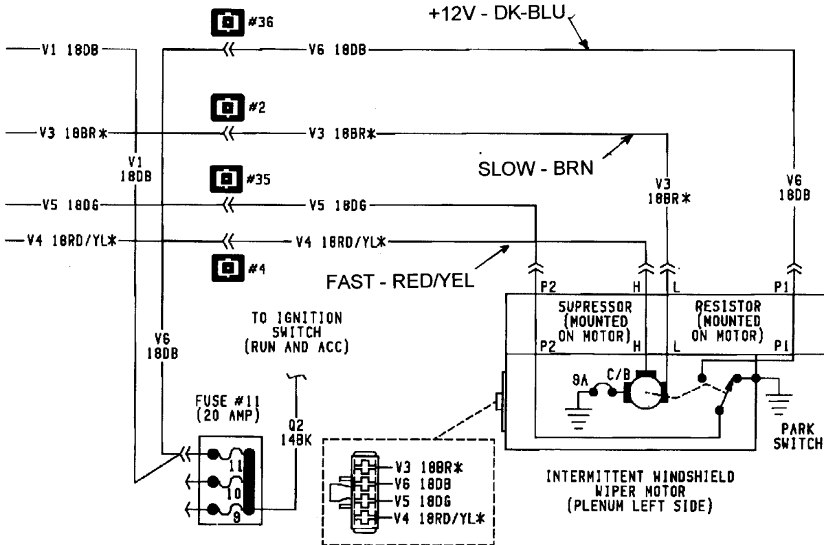
Wiper & Washer System Wiring Circuit (Front) -- Part 2
