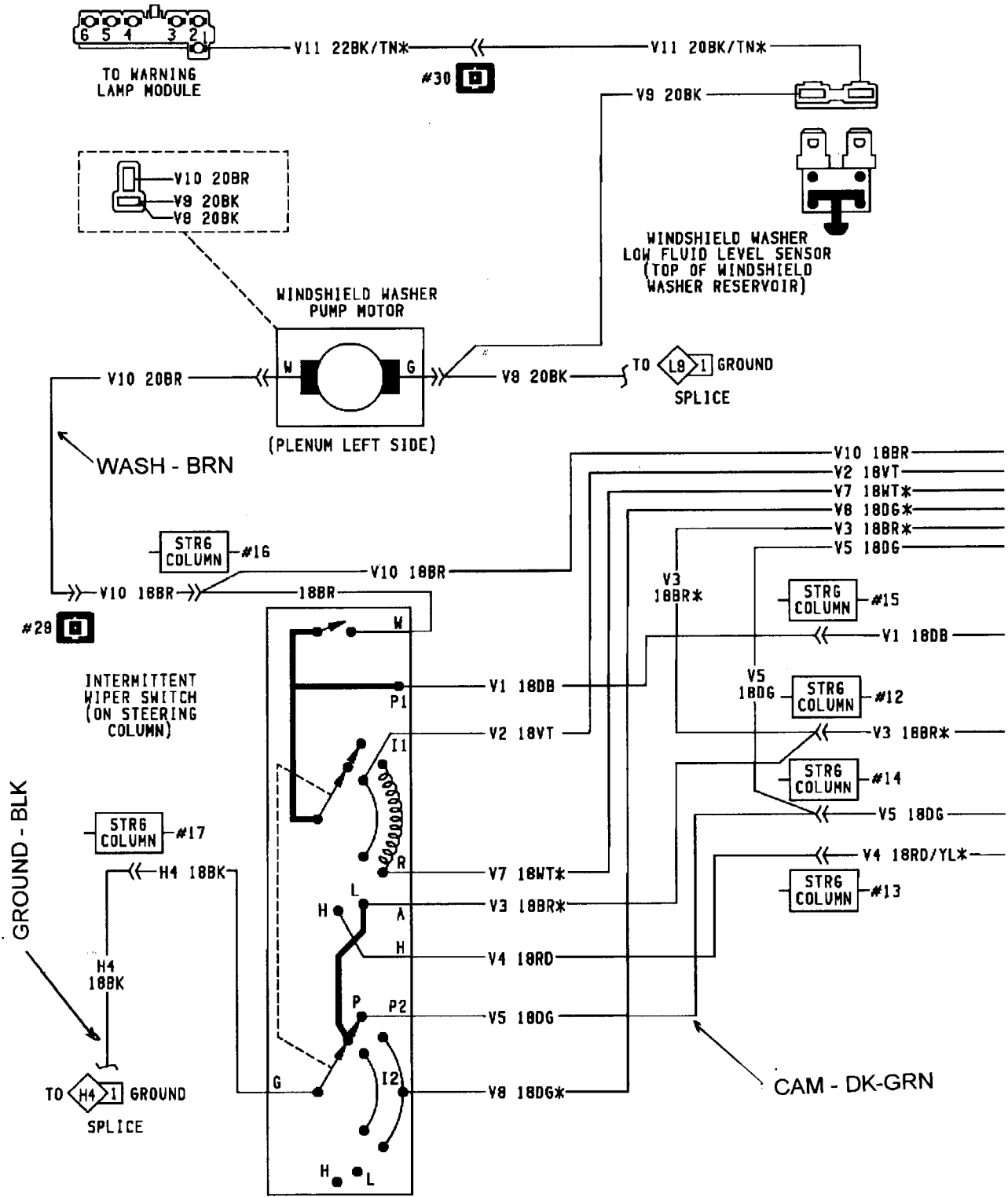
Wiper & Washer System Wiring Circuit (Front) -- Part 1
