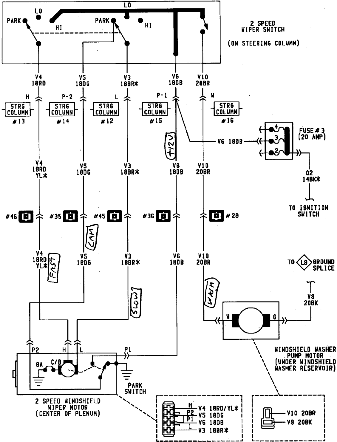
Windshield Wiper System Wiring Circuit. Less Intermittent
