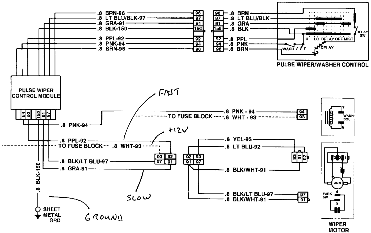
Wiper/Washer Wiring Circuit. With Pulse
