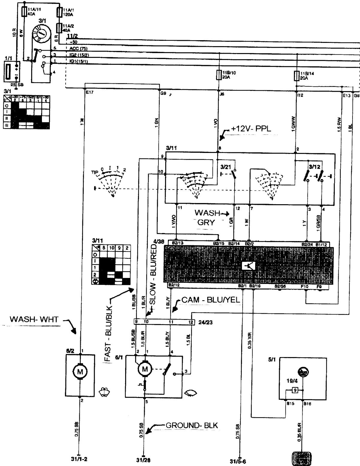
Windshield Wiper And Windshield Washer, Part 1 Of 2
