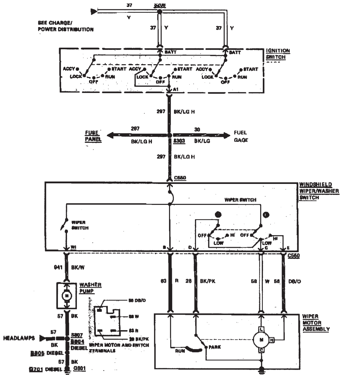
Fig. 133 Windshield wiper & washer wiring circuit. 1984 Bronco & F100-350 less intermittent wipers
