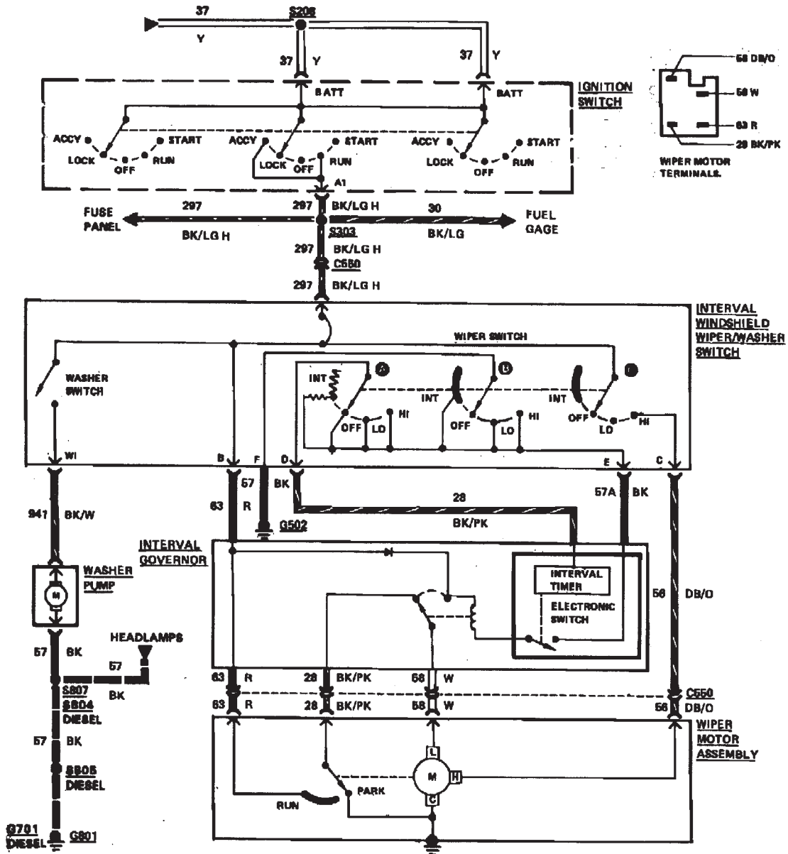
Fig. 134 Windshield wiper & washer wiring circuit. 1984 Bronco & F100-350 with intermittent wipers
