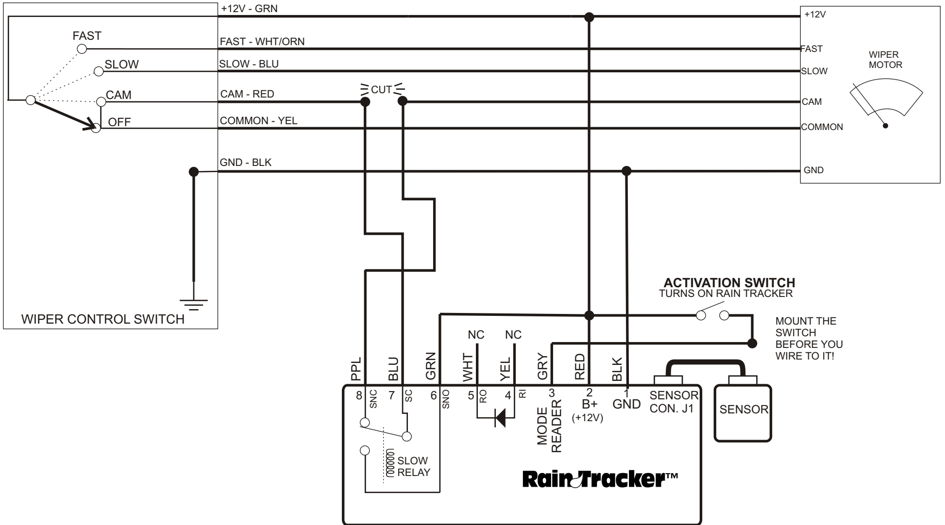
RAIN TRACKER INTERFACE WIRING DIAGRAM WIPER SYSTEM CLASS: Ford-Truck Econoline w/o Factory Intermittent
