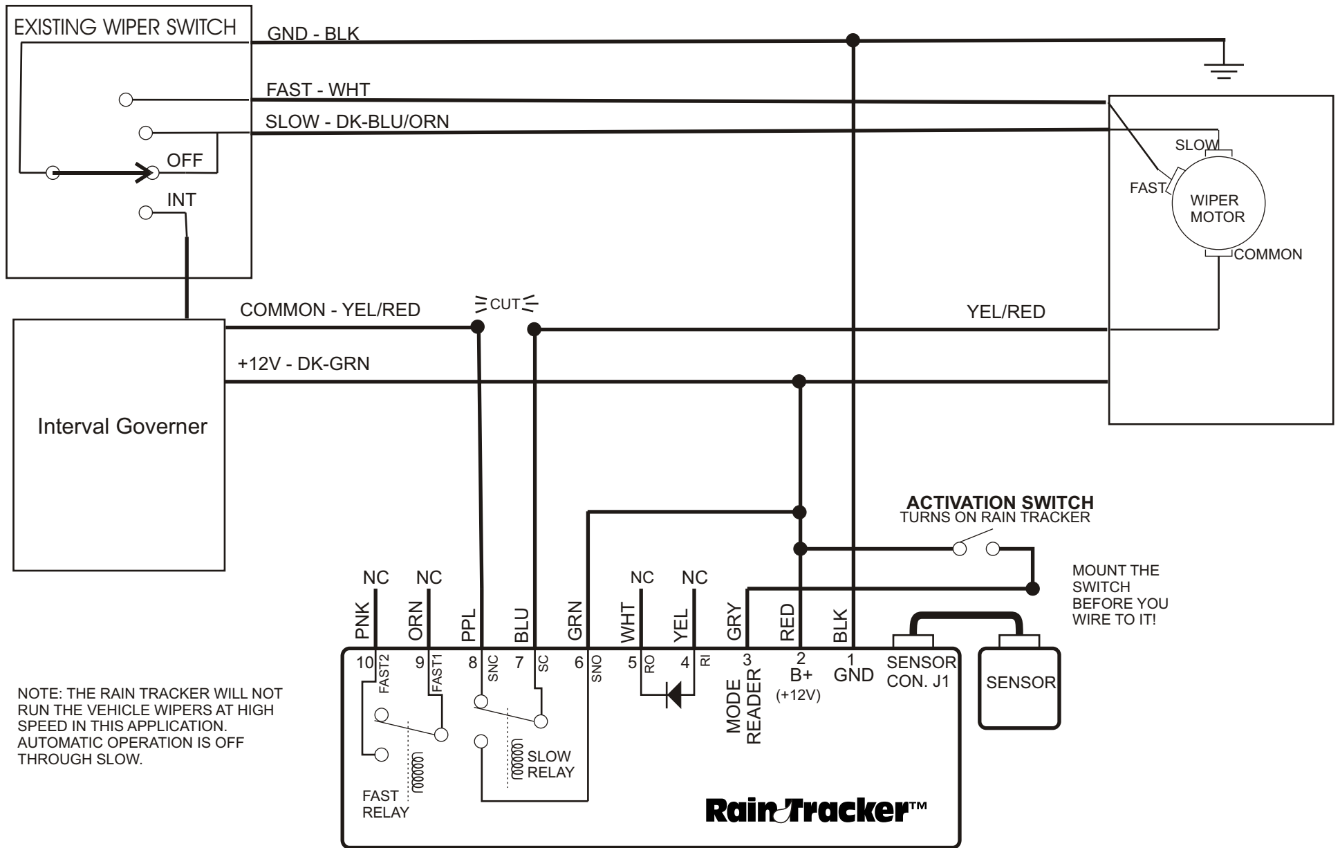
RAIN TRACKER INTERFACE WIRING DIAGRAM WIPER SYSTEM CLASS: Ford E-150 VAN
