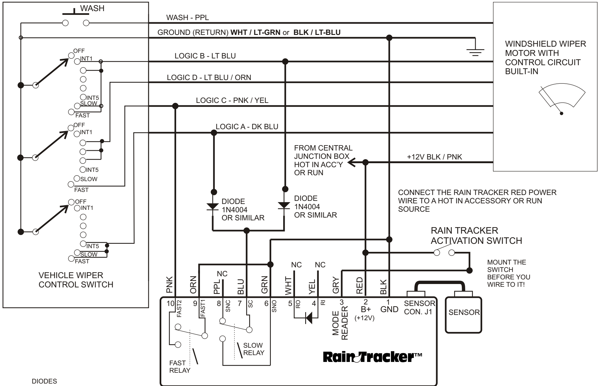
RAIN TRACKER INTERFACE WIRING DIAGRAM WIPER SYSTEM CLASS: Ford BINARY - C1 FORD BINARY STYLE WITH WIRE-COLOR SCHEME 1
