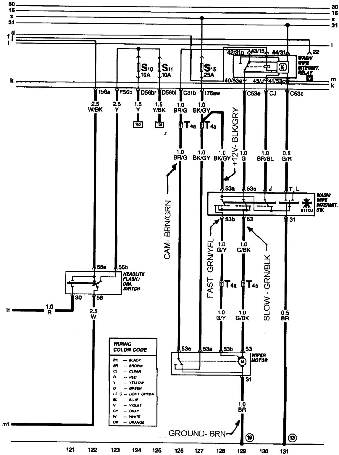
Windshield Washer/Wipers. Wiring Diagram
